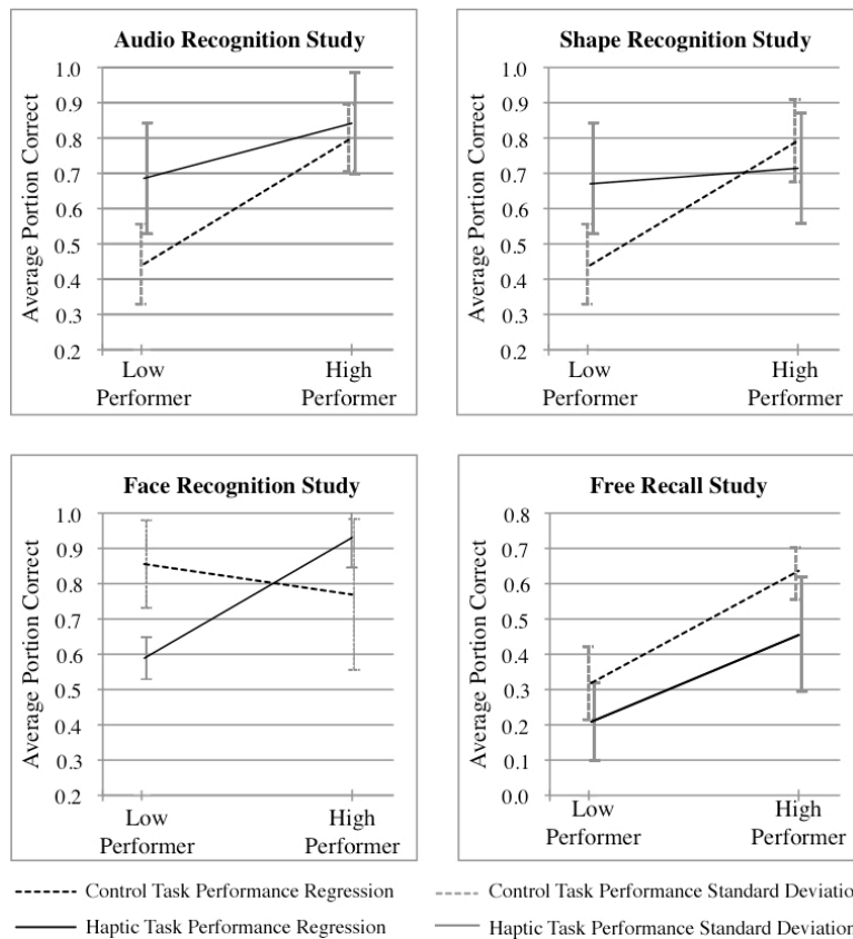
Fig. 2. Performance on shape, face, and audio recognition tasks with haptic cues interacts with performance on the control tasks ( p < 0.001 , p < 0.001 , p = 0.0239 respectively). Free recall shows no significant interaction, as both types of users performed consistently worse.
